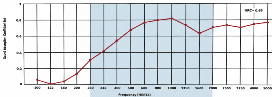
ACUSTA - CORDELIA - ACOUSTIC TEST RESULTS / REVERBERATION ROOM METHOD / EN ISO 354:2007-02 (10 cm. distance from wall)
